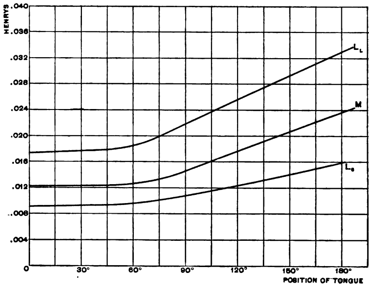
FIG. 2.—Variation of Constant.
